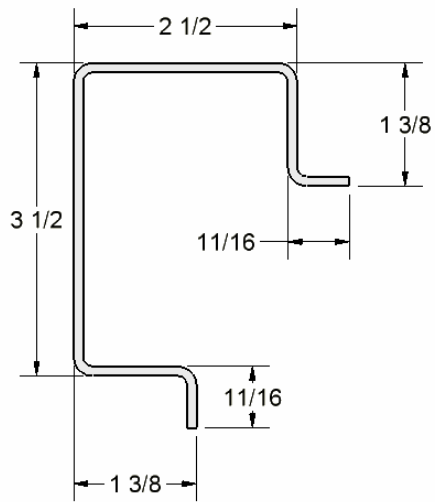
PART 5314 CORNER POST 12 GA.
