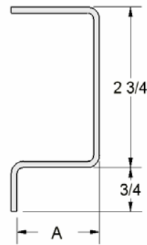
PART 5048 DOOR HEADER 12 GA. A = 1 1/4", 1 1/2", OR 1 3/4"
