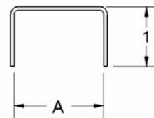
PART 5069 LINTEL—16 GA. A = 1 1/4", 1 1/2", OR 1 3/4"
