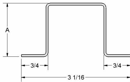
PART 5055 BODY POST 16 GA. A = 1 1/4", 1 1/2", OR 1 3/4"
