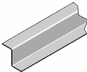
PART 5055 BODY POST 16 GA. A = 1 1/4", 1 1/2", OR 1 3/4"
