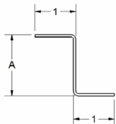
PART 5070 ZEE POST 16 GA. A = 1 1/4", 1 1/2", OR 1 3/4"
