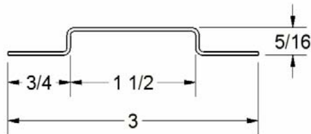
PART 5128 SINGLE BELT RAIL 19 GA.
