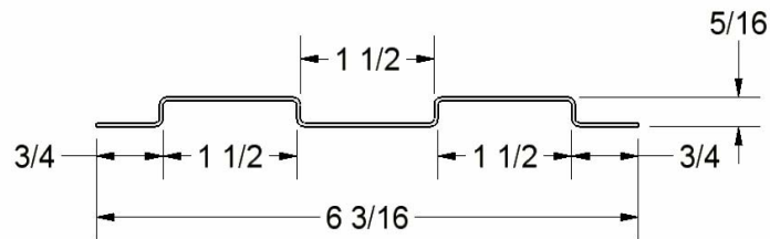
PART 5222 DOUBLE BELT RAIL 19 GA.
